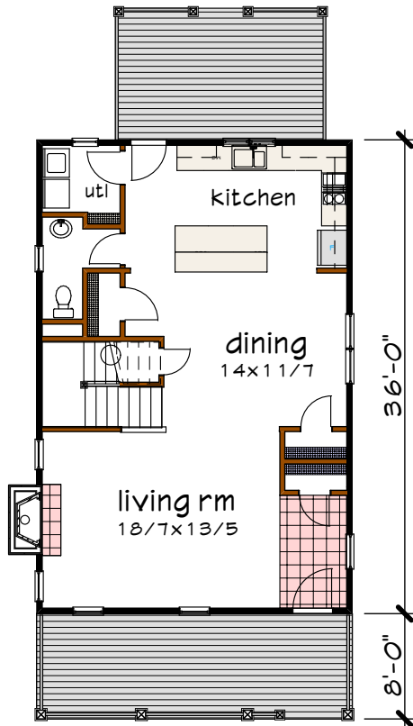
Floor 1 plan
