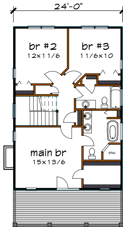
Floor 2 plan
