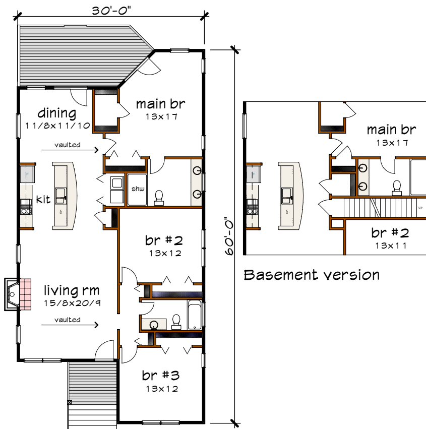
Floor 1 plan
