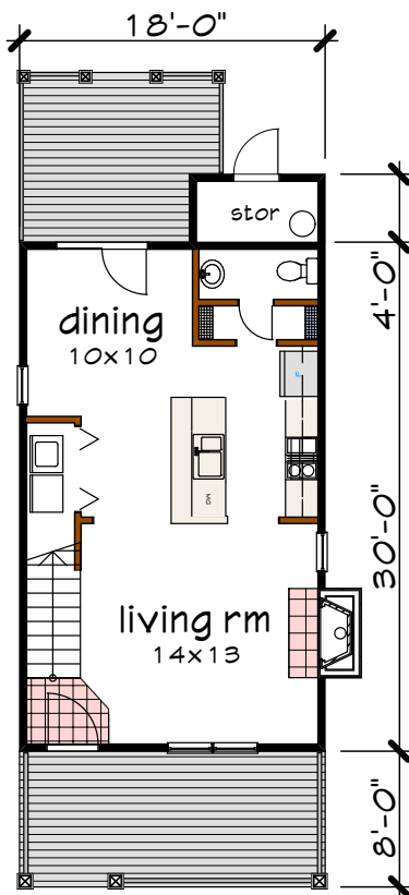
Floor 1 plan
