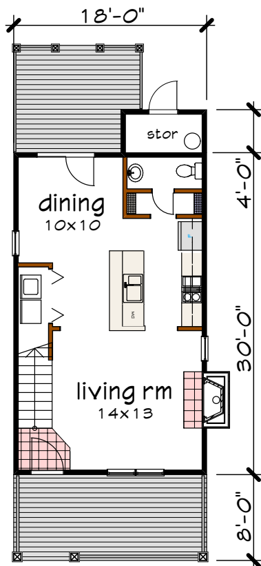
Floor 1 plan
