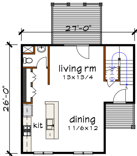
Floor 1 plan
