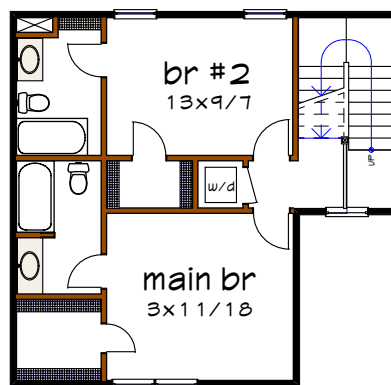
Floor 2 plan
