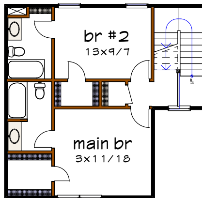
Floor 2 plan
