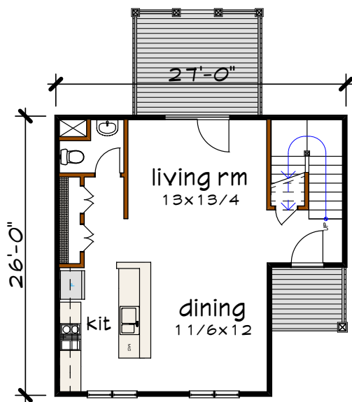
Floor 1 plan
