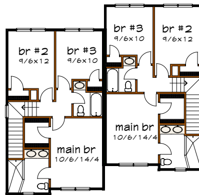
Floor 2 plan
