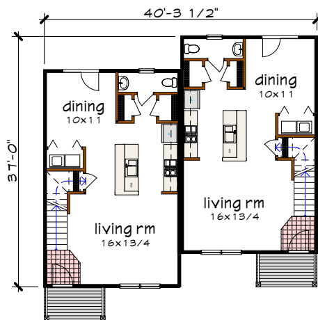
Floor 1 plan
