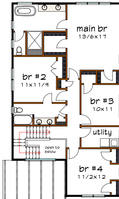
Floor 2 plan
