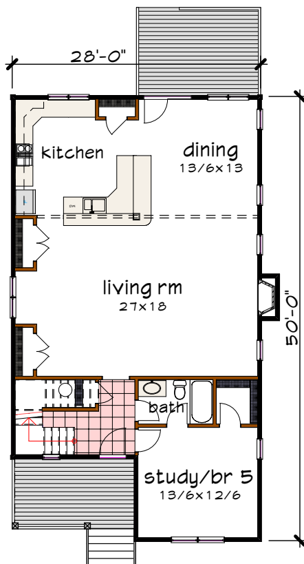
Floor 1 plan
