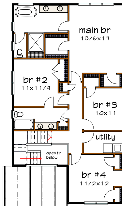
Floor 2 plan
