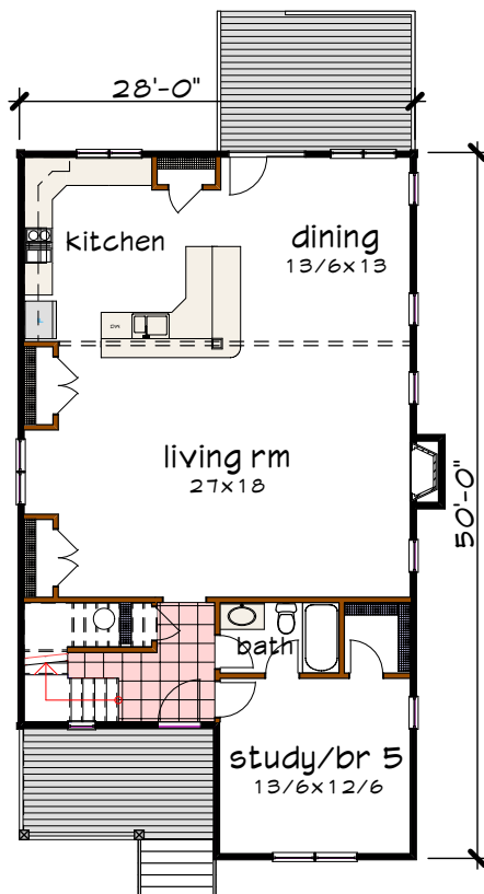
Floor 1 plan
