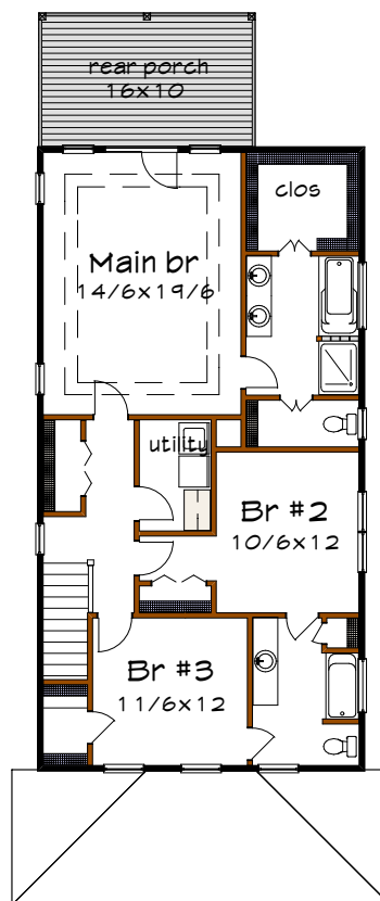
Floor 2 plan
