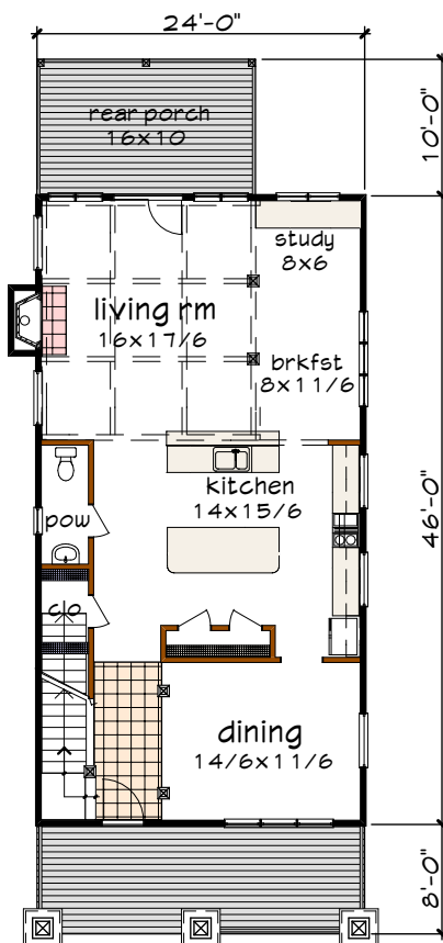
Floor 1 plan
