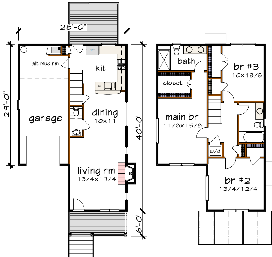
Floor 1 plan
