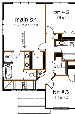
Floor 1 plan
