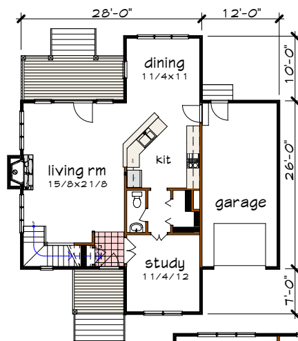
Floor 1 plan
