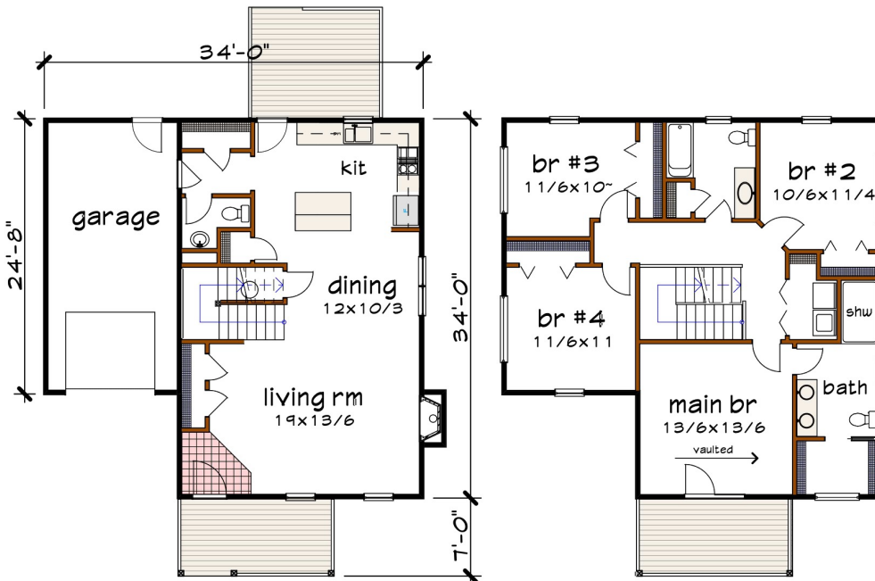
Floor 1 plan
