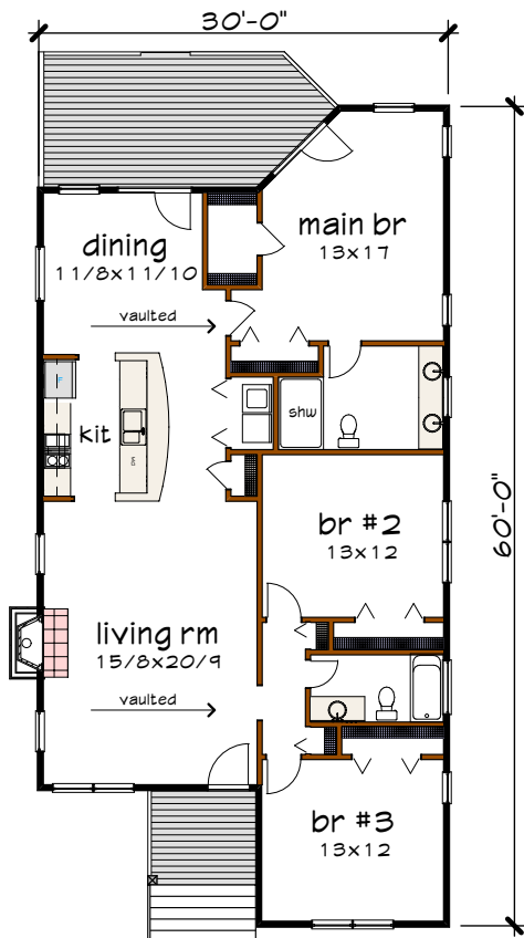
Floor 1 plan
