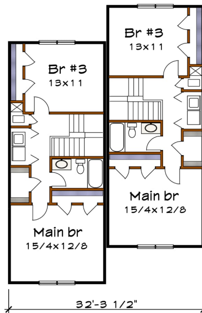
Floor 2 plan
