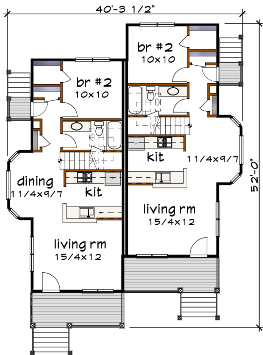
Floor 1 plan
