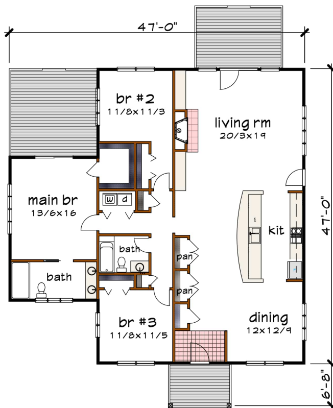
Floor 1 plan
