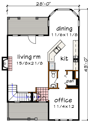
Floor 1 plan
