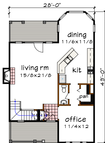
Floor 1 plan
