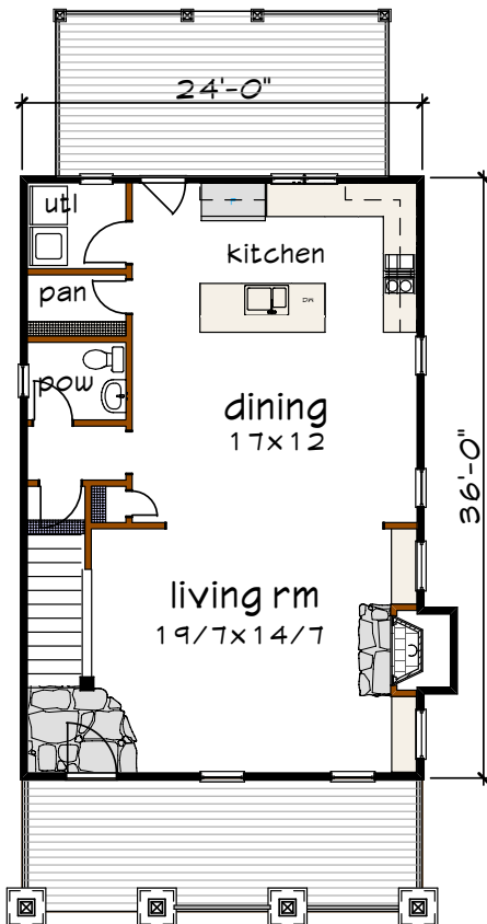
Floor 1 plan
