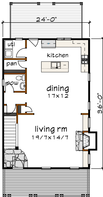
Floor 1 plan
