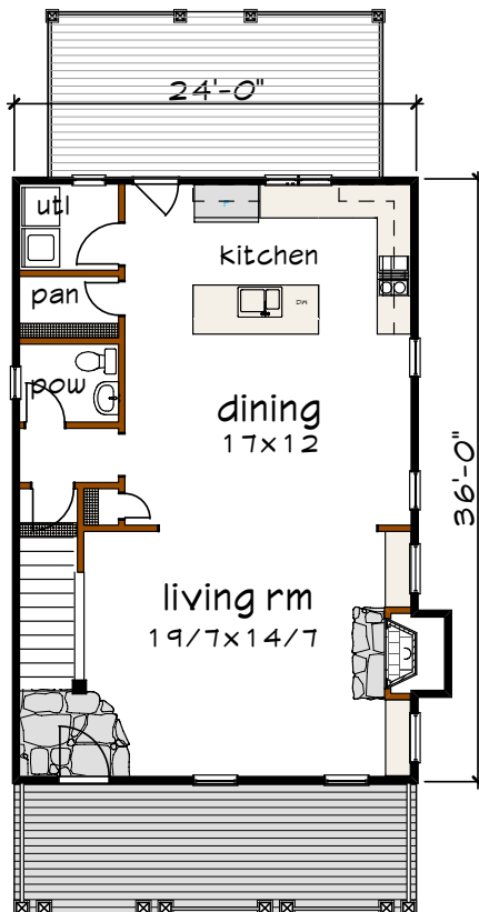
Floor 1 plan
