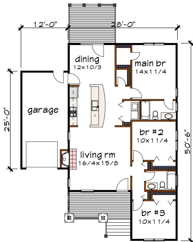
Floor Plan
