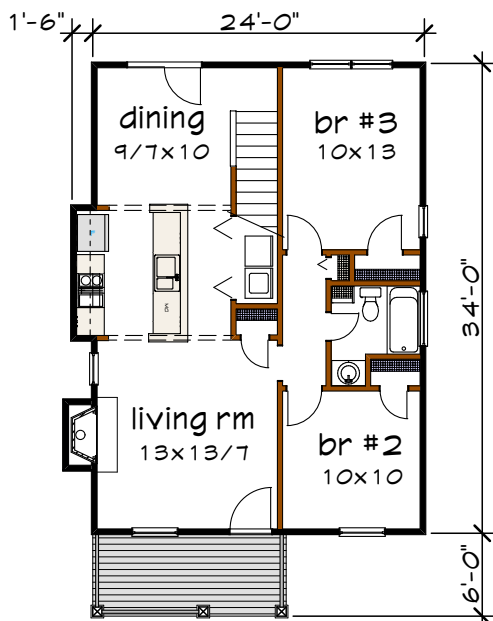
Floor 1 plan
