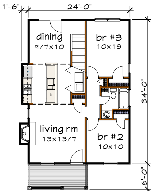
Floor 1 plan
