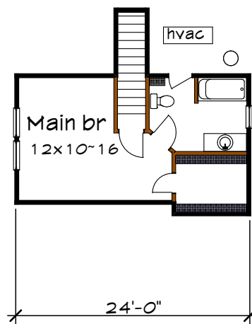
Floor 2 plan
