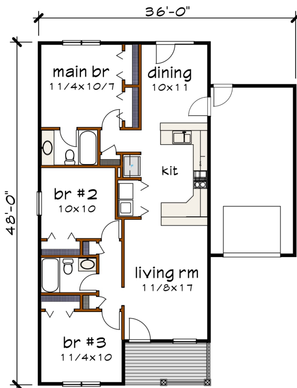
Floor Plan
