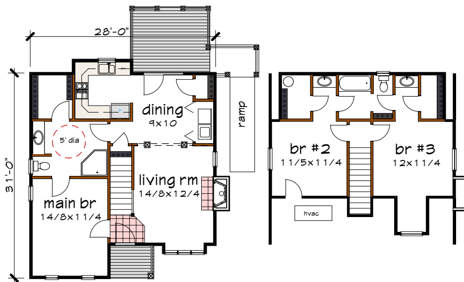
Floor 1 plan
