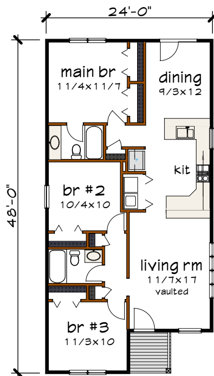
Floor 1 plan
