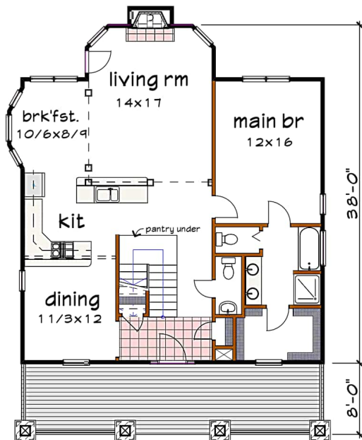
Floor 1 plan
