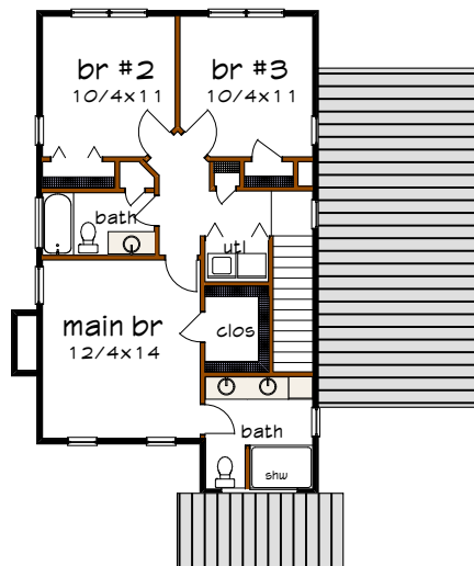
Floor 2 plan
