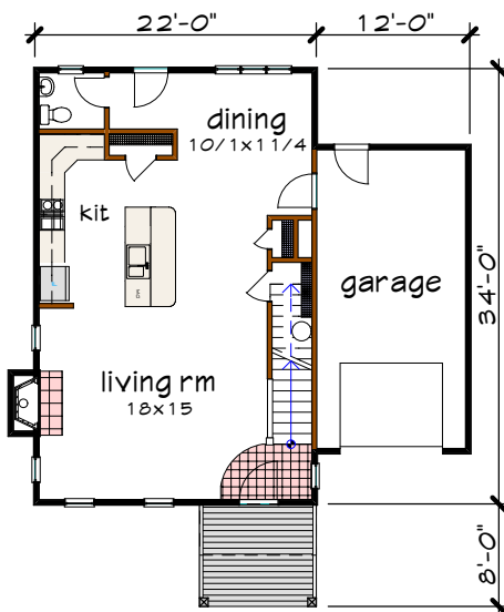
Floor 1 plan
