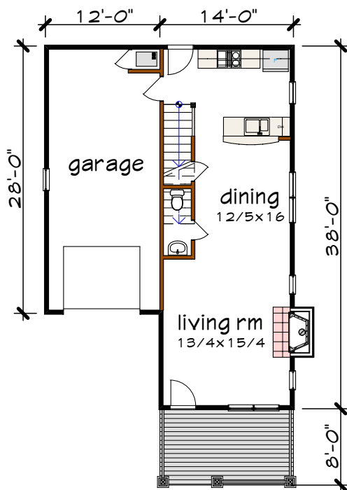
Floor 1 plan
