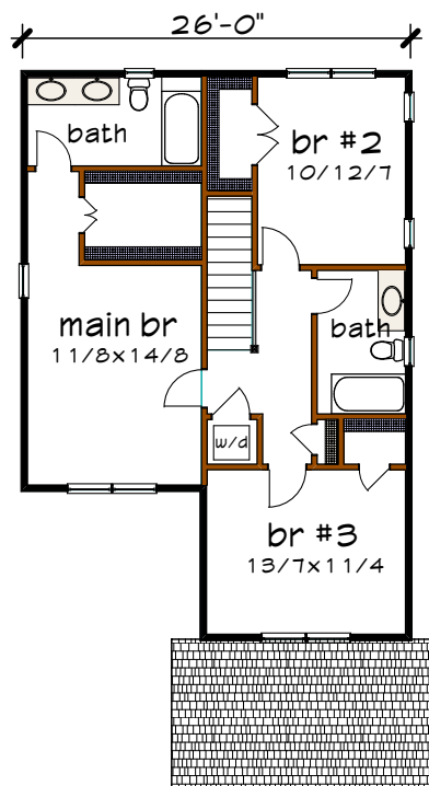
Floor 2 plan
