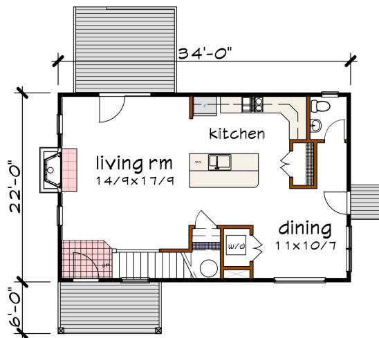
Floor 1 plan
