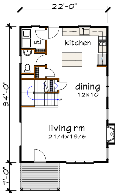
Floor 1 plan
