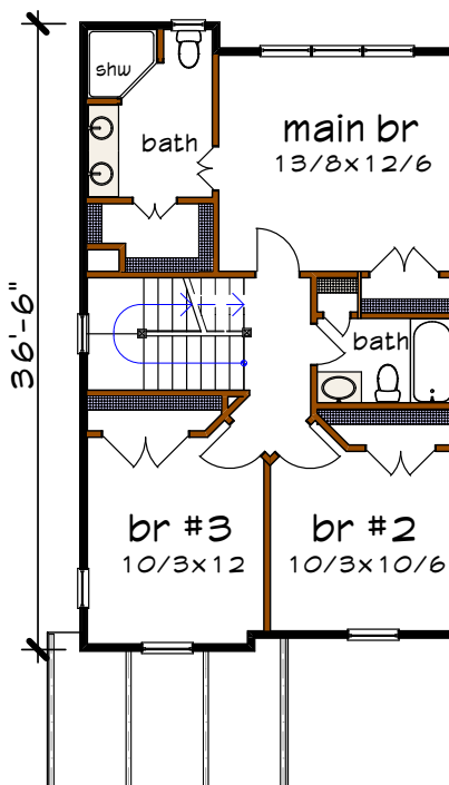
Floor 2 plan
