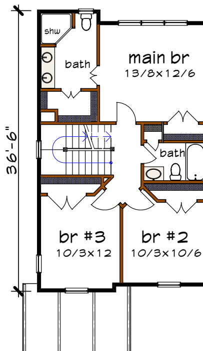
Floor 2 plan
