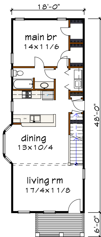
Floor 1 plan
