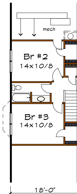
Floor 2 plan
