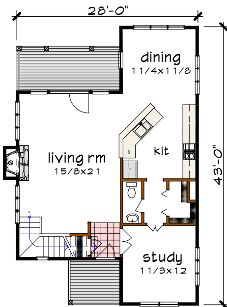
Floor 1 plan
