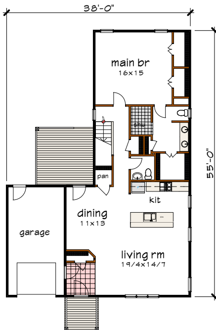
Floor 1 plan
