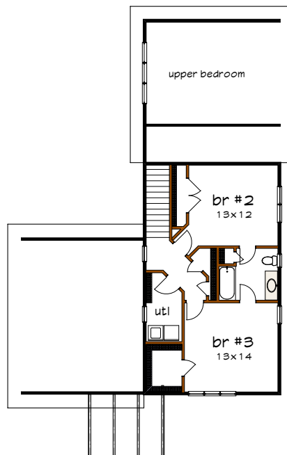
Floor 2 plan
