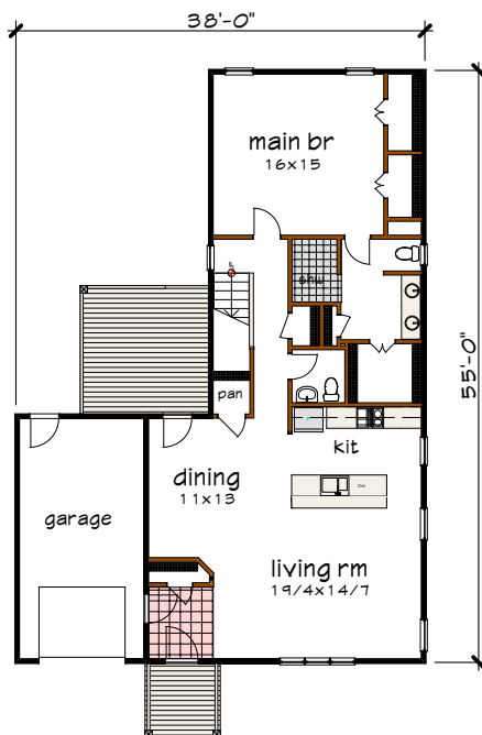
Floor 1 plan
