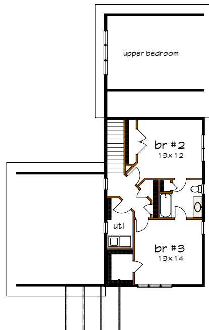
Floor 2 plan
