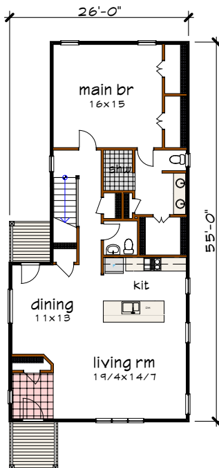
Floor 1 plan
