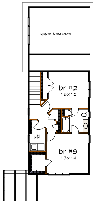
Floor 2 plan
