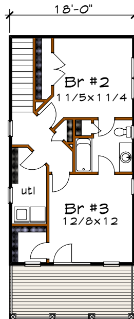
Floor 2 plan
