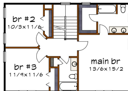
Floor 2 plan
