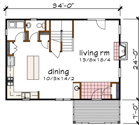
Floor 1 plan
