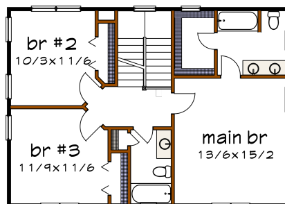
Floor 2 plan
