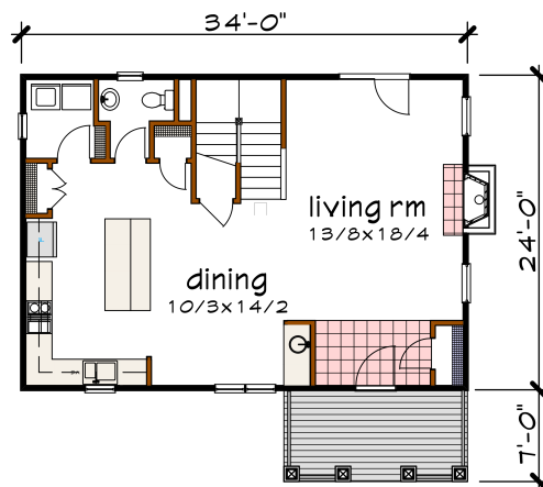
Floor 1 plan
