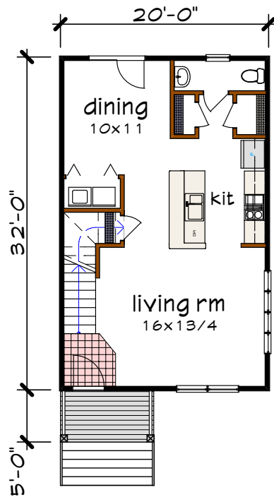
Floor 1 plan
