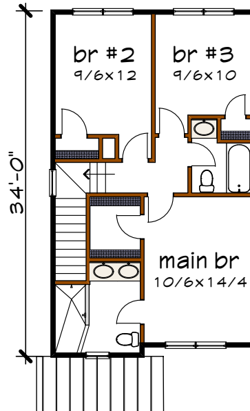
Floor 2 plan
