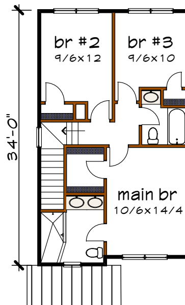
Floor 2 plan
