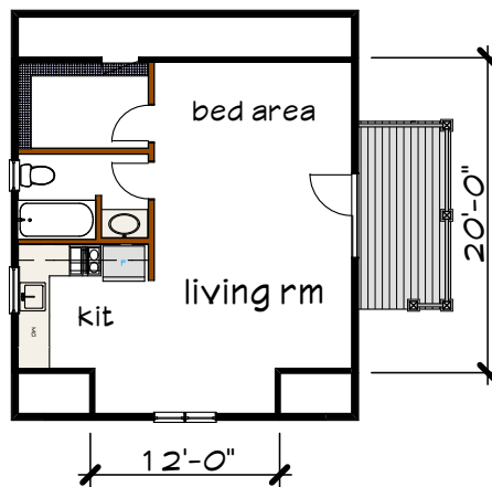
Floor 2 plan
