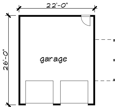
Floor 1 plan
