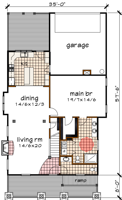
Floor 1 plan
