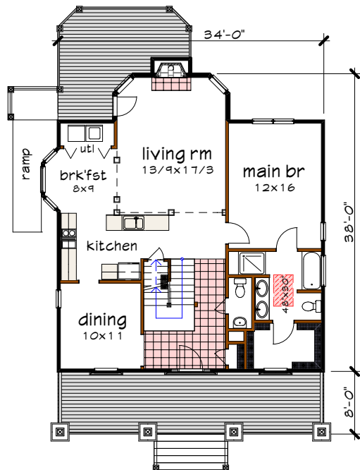
Floor 1 plan
