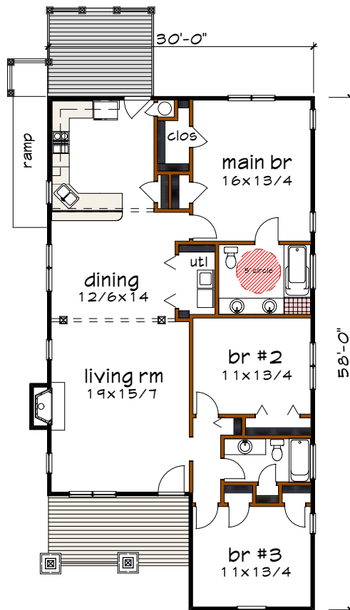
Floor plan
