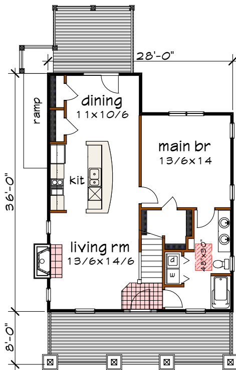
Floor 1 plan
