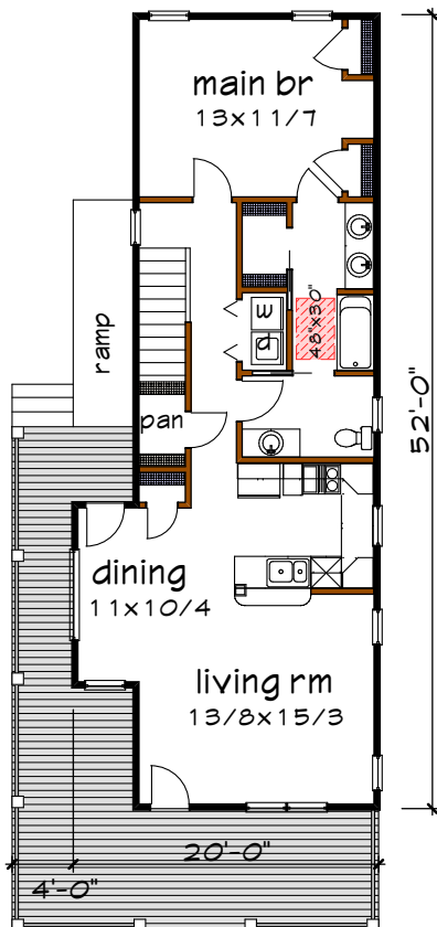
Floor 1 plan
